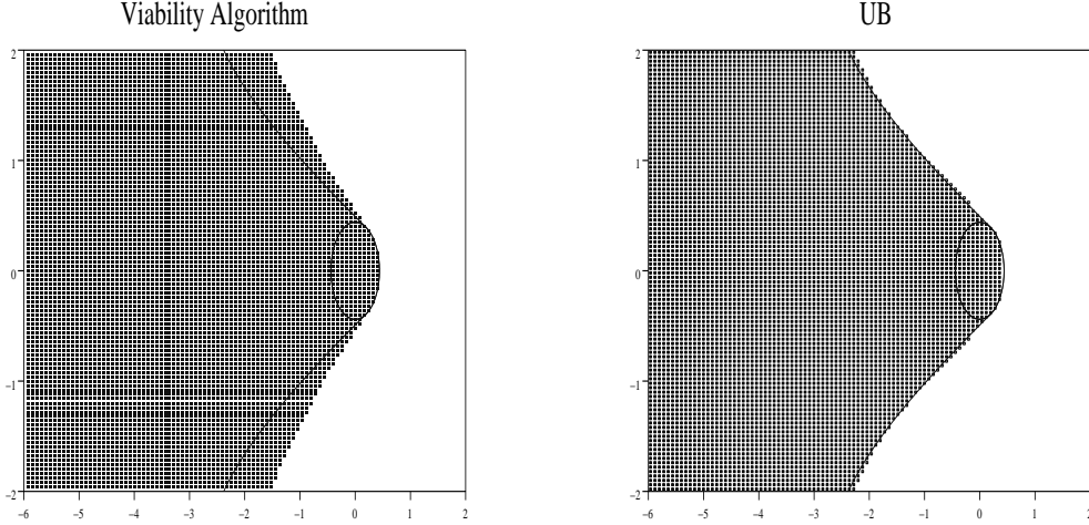
Figure 2: Approximation of the capture basin for the zermelo problem, P_{x_1} = P_{x_2} = 100
