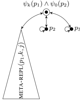
Fig. 18: The action e_M(k, l, m) when I_k = \text{jzdec}(0, j), l = 0 . Case I_k = \text{jzdec}(1, j), m = 0 is by replacing p_2 with p_3 .
