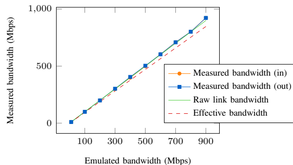
Figure 7. Emulation of high-bandwidth network link.
