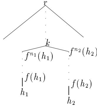
Figure 8: Factorization
