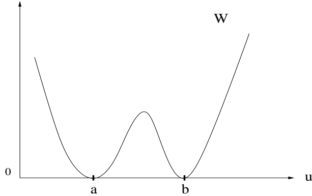
Figure 2: Example of double-well potential W .
