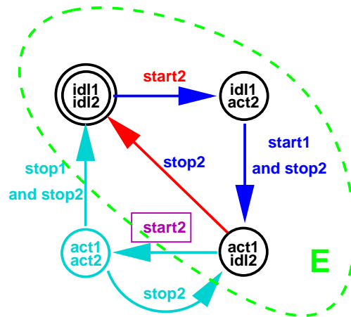
Figure 8: Controlled behaviours of a 2-tasks system.
