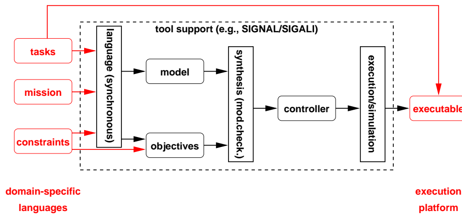
Figure 15: Integration of discrete control synthesis into an automated process.
