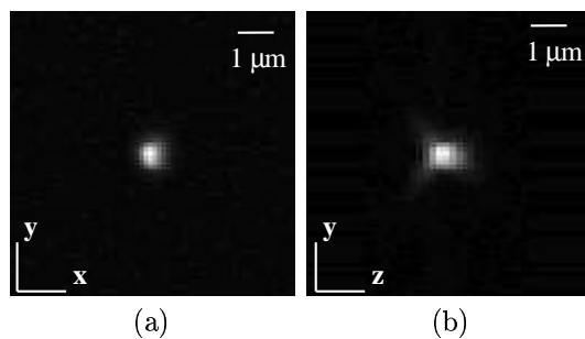
Figure 3: An approximation of the real PSF. Two views of the image of a small bead of diameter 175 nm: (a) is the lateral XY view, (b) the axial XZ view. Initially, the size of a voxel is 89 \times 89 \times 230 nm in X , Y and Z . In the figure, it is now 89 nm in each of the three directions. Note that there was no resampling. This is the best approximation we have to illustrate the real PSF; the lateral size is 491 nm (6 pixels). and the axial size is 1150 nm. A good estimation of the size of the PSF is to remove this approximate size of 175 nm of the bead, that gives a PSF with a size of 316 nm in XY and 975 nm in XZ .
