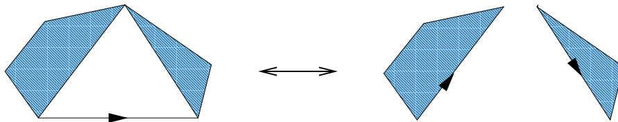
FIGURE 8. Bijection entre \mathcal{P}_1 et \mathcal{P}^2 .
