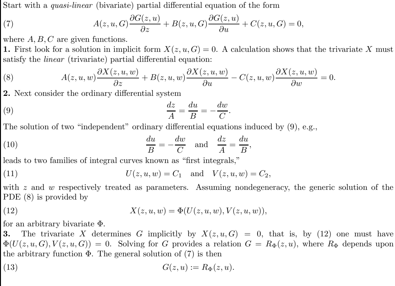
FIGURE 1. The solution algorithm for quasilinear PDEs of first order.
