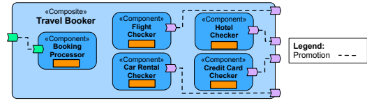
Figure 4. A travel booker implementation with the SCA.
