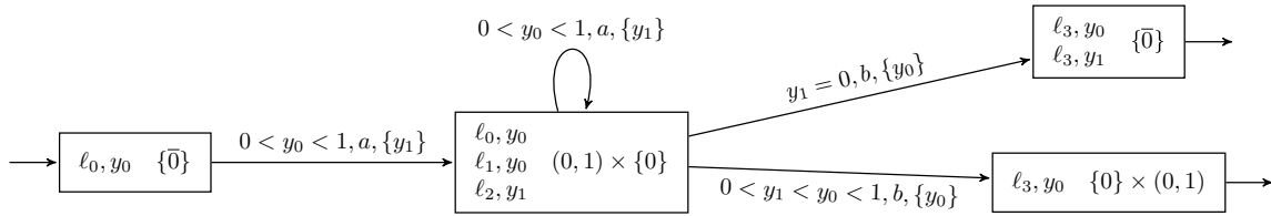
Figure 7: The result of procedure [BBBB09a] on the running example.
