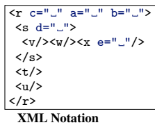
Figure 4. Sample XML Tree with Attributes.
