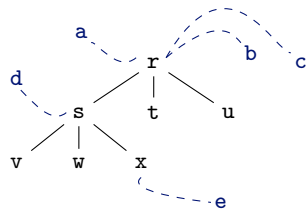
Figure 4. Sample XML Tree with Attributes.
