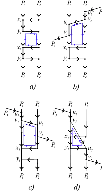
FIGURE 3 – Helly property
