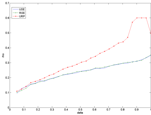
Fig. 9. Observed Phase Transition of Recommended IST for different matrix ensembles.
