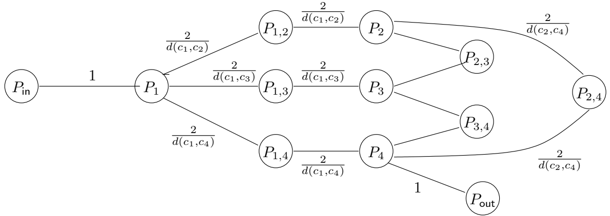
Figure 5: The platform used in the reduction for Theorem 4.
