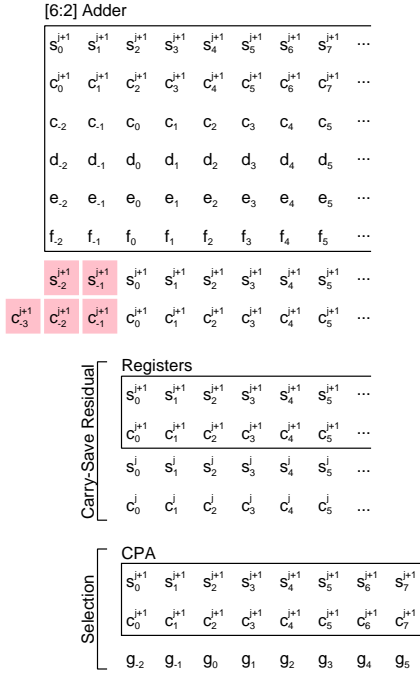
Fig. 7. First implementation of recurrence reduction. Each rectangular box represents some functional block where the bits inside show the inputs to that block and the bits beneath show the corresponding outputs. There are 5 bits produced by the [6 : 2] adder in this figure which have a shaded square background to signify that these output bits don't drive any logic and are left "open".
