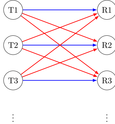
Figure 1: K -users interference channel. The first 3 transmitter-receiver pairs are represented on this figure. The blue lines indicate the desired links, whereas the red lines indicates the interfering links.
