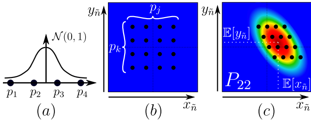
Figure 6: Sampling distribution P_{22} . (a) We precompute uniform 1D samples p_j . (b) In the fragment shader we compute the Cartesian product and get 2D samples (p_j, p_k) . (c) We scale, correlate, and shift the samples to match distribution P_{22} .
