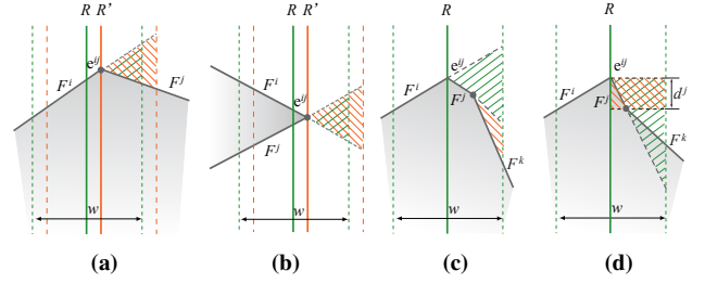
Figure 3: blue 2D Volume approximation. In each figure, a solid vertical line represents a ray, and dotted lines of the same color mark the extent of the ray volume. F , e are face and edge’s 2D representation. Each volume error created by an edge e^{ij} is highlighted with a hatched polygon with the same color as the ray. (a): The volume is maximum (in red) when the ray crosses the edge. (b): This also holds for silhouette edges. (c): Multiple edge volumes (red, green) are summed up. (d): Narrow face volumes are more tightly bound by rectangles (red) than by triangles (green).
