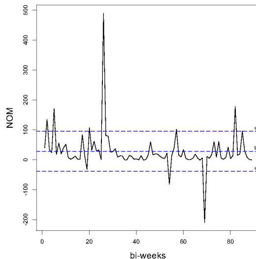
Figure 2. NOM series in first difference (stationary behaviour)
