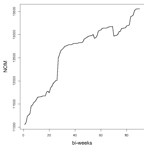
Figure 1. Original NOM series (non-stationary behaviour)
