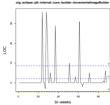
Figure 4. Example of non-stationary time series
