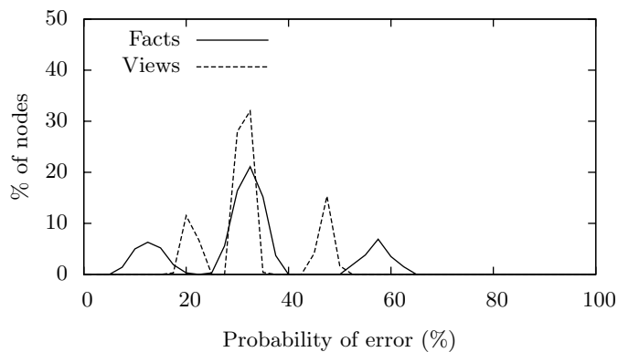
Figure 1: Distribution of errors on synthetic dataset
