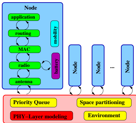
Fig. 5. The WSNnet simulation environment.
