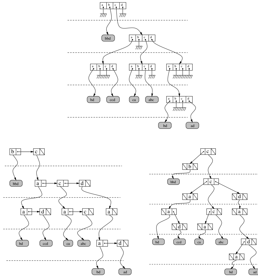
FIGURE 3. Three representations of a trie built from the sequence of words (cccabc, bbbd, cdadad, ccaca, caabd, cadccd, cdaabd) over the alphabet \mathcal{A} = \{a, b, c, d\} : the array-trie (top; the null pointers are represented as electrically grounded), the list-trie (bottom left) and the bst-trie (bottom right).
