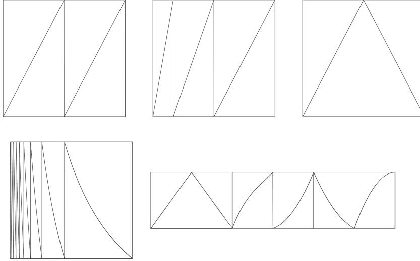
FIGURE 1. Five dynamical sources. From top to bottom: (a) binary representations; (b) a memoryless source with probabilities (\frac{1}{6}, \frac{1}{3}, \frac{1}{2}) ; (c) the binary reflected code; (d) continued fraction representations; (e) a Markov source (S_0, S_1, S_2) that switches between two different representations. The plots represents the graphs of the associated shifts T .
