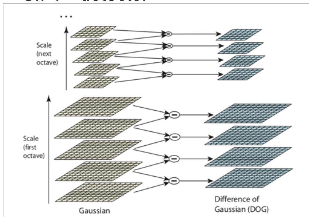
DoG computation
