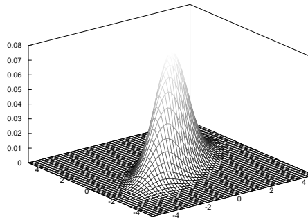
Figure 8.2: 2-D Gaussian pdf
