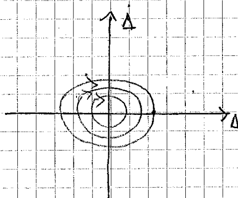
phase portrait
